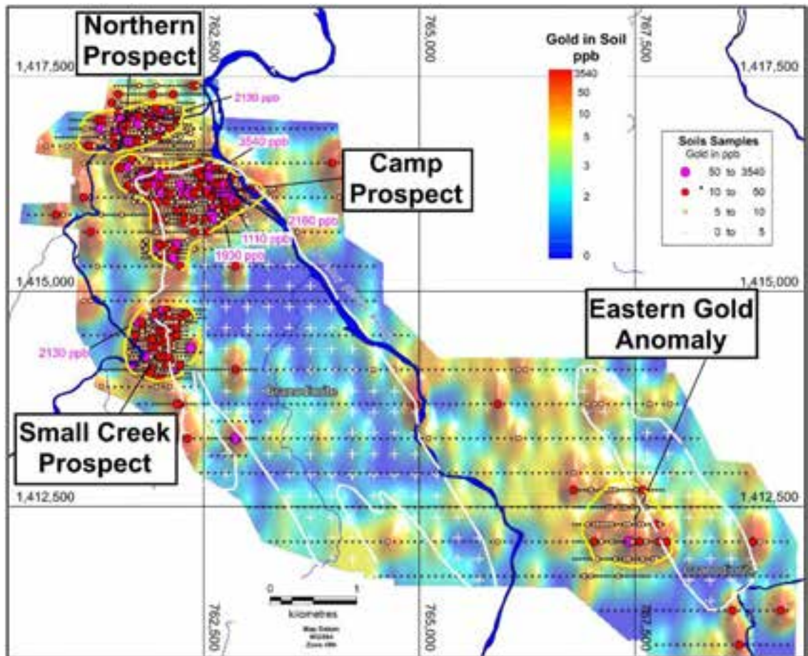
Figure 14. Soil sample locations and gold results at O'Phay Gold Project over the imaged gold-in-soil assay data (inverse distance method).
