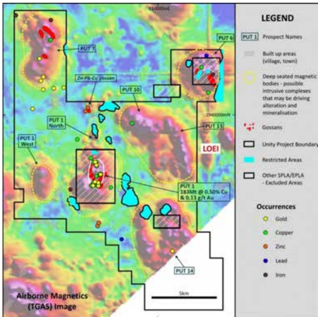
Figure 17. Unity Metals' Loei Copper Gold Project area in northern Thailand with prospect locations and gold occurrences over an airborne magnetic image.
