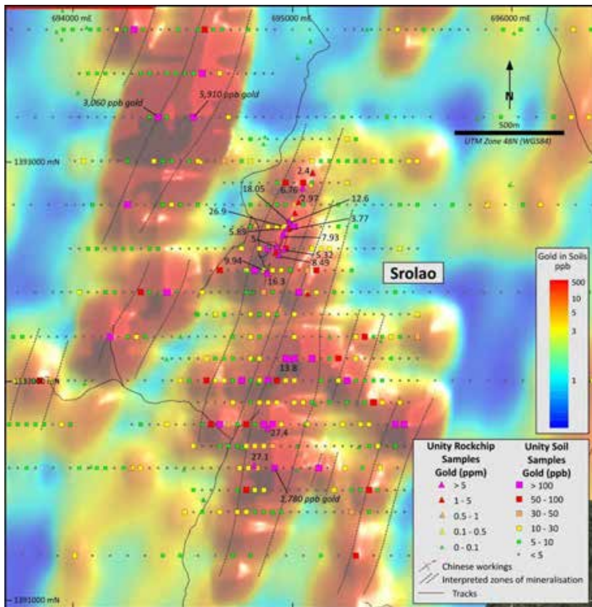
Figure 11. Srolao Gold Prospect. Soil and rock chip sample results on gridded gold-in-soil image.
