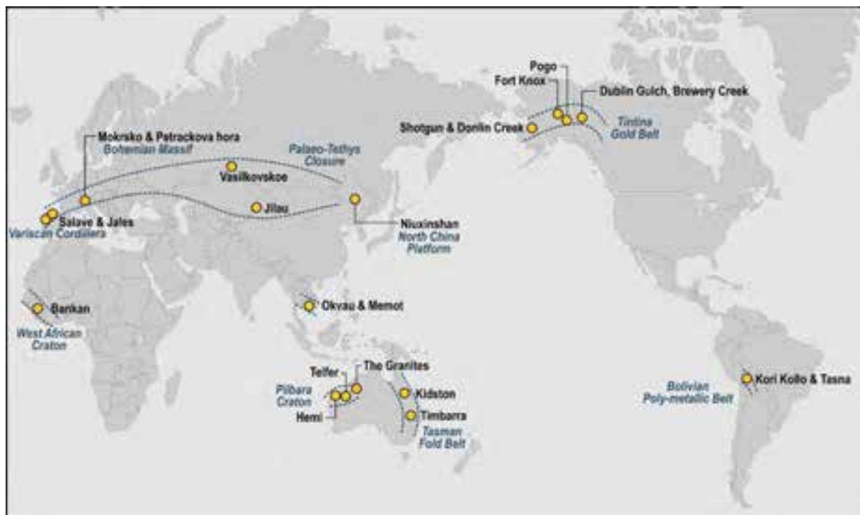
Figure 6: Worldwide distribution of major intrusion related gold deposits. Source: Unity Metals. Modified from Lang and Baker, 2001.
