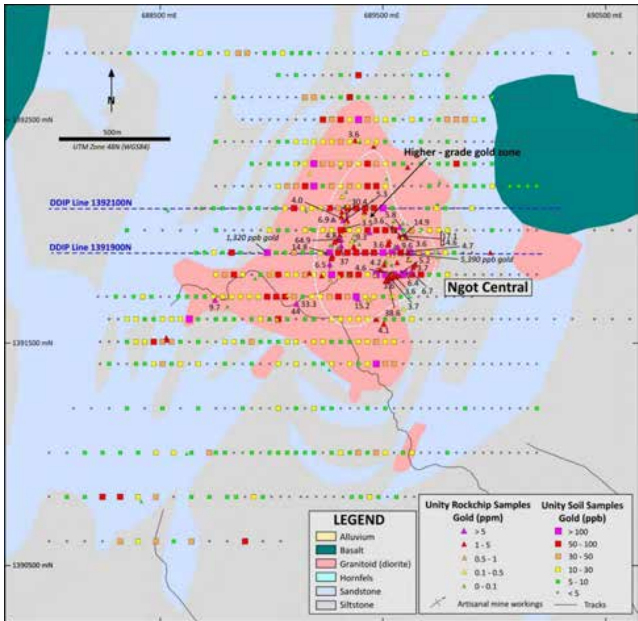
Figure 19: Ngot Central Prospect. Soil and rock chip sample results on geology, location of IP lines shown. Source: Unity Metals.
