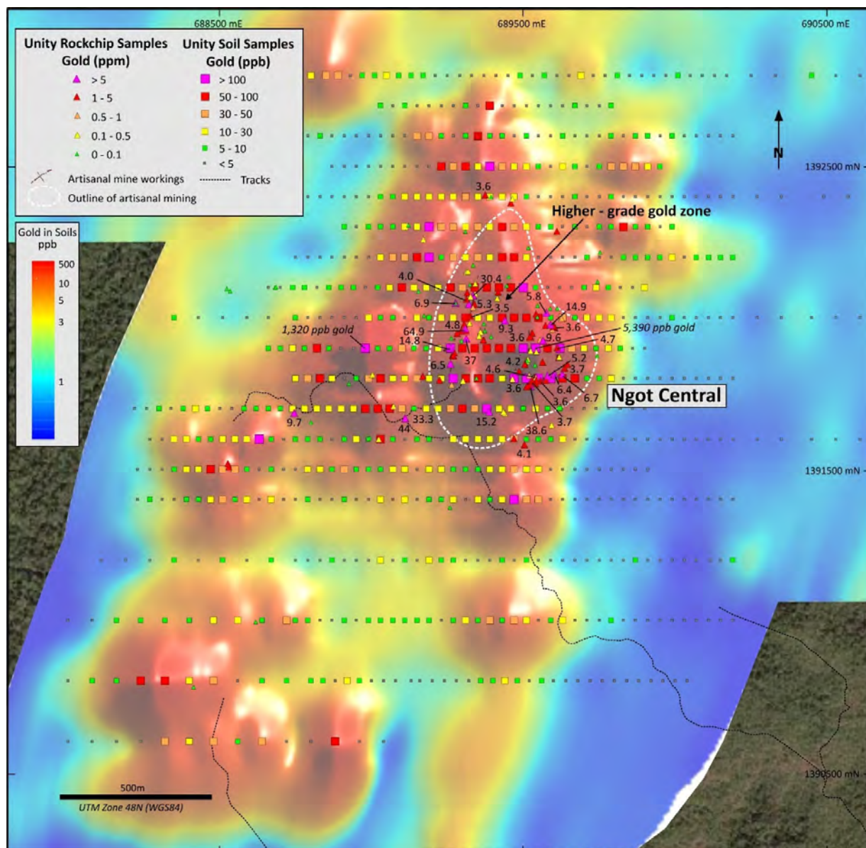
Figure 20. Ngot Central Prospect. Soil and rock chip sample gold results on a gridded gold-in-soil image. Source: Unity Metals.
